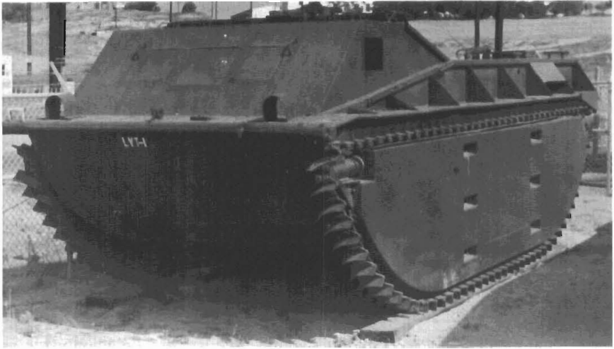
LVT-1 (1941)
